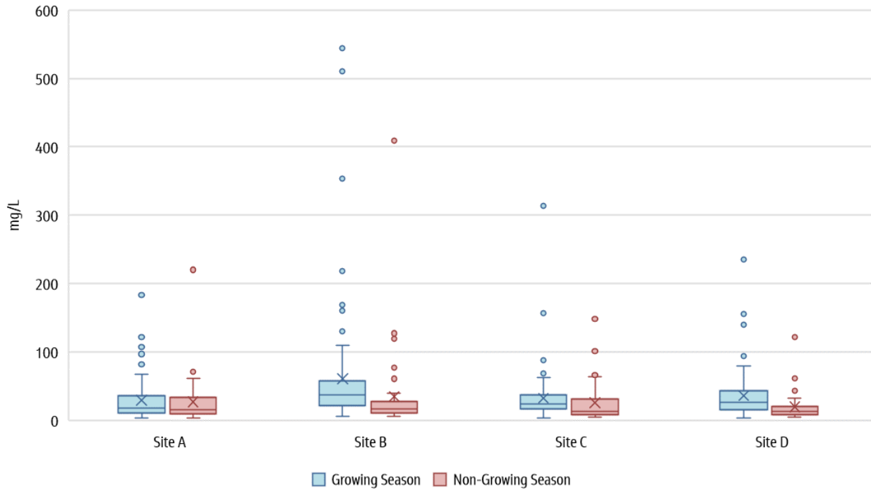
Figure 5-11. Total Suspended Solids Box and Whisker Plot by Site and Season
