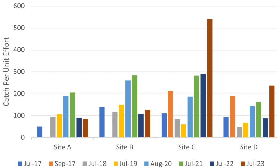
Figure 6-2. Summer Fish Survey Catch Per Unit Effort
