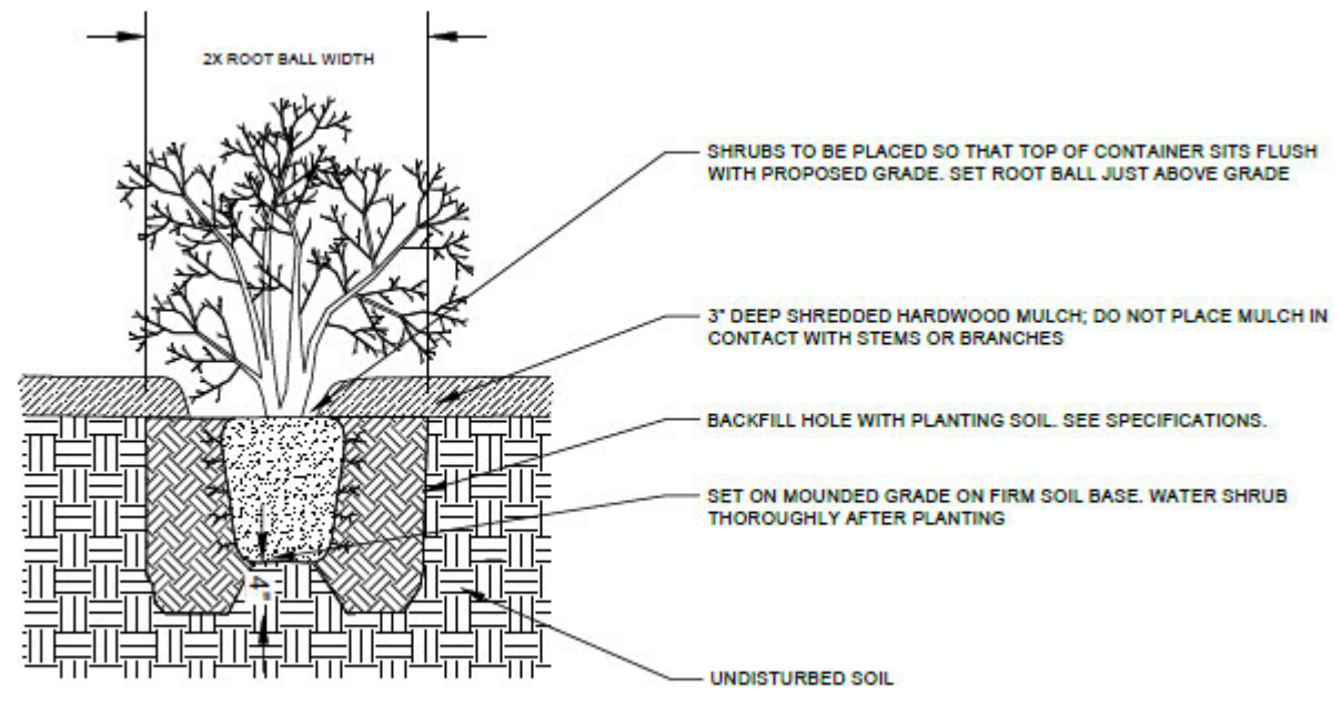
01 DECIDUOUS SHRUB PLANTING 34 NOT TO SCALE
