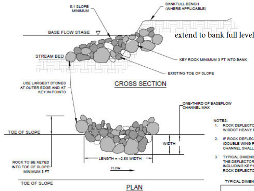
03 ROCK DEFLECTOR 33 NOT TO SCALE
