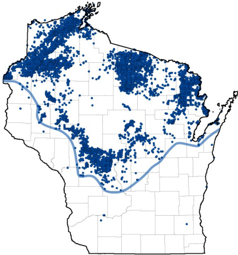
Figure 32.5. Map of red pine distribution from the GLO PLS data. A general range line for red pine in Wisconsin in the mid-1800's has been estimated and inserted to delimit the common occurrence of red pine; community outliers did sporadically occur beyond these range limits.
