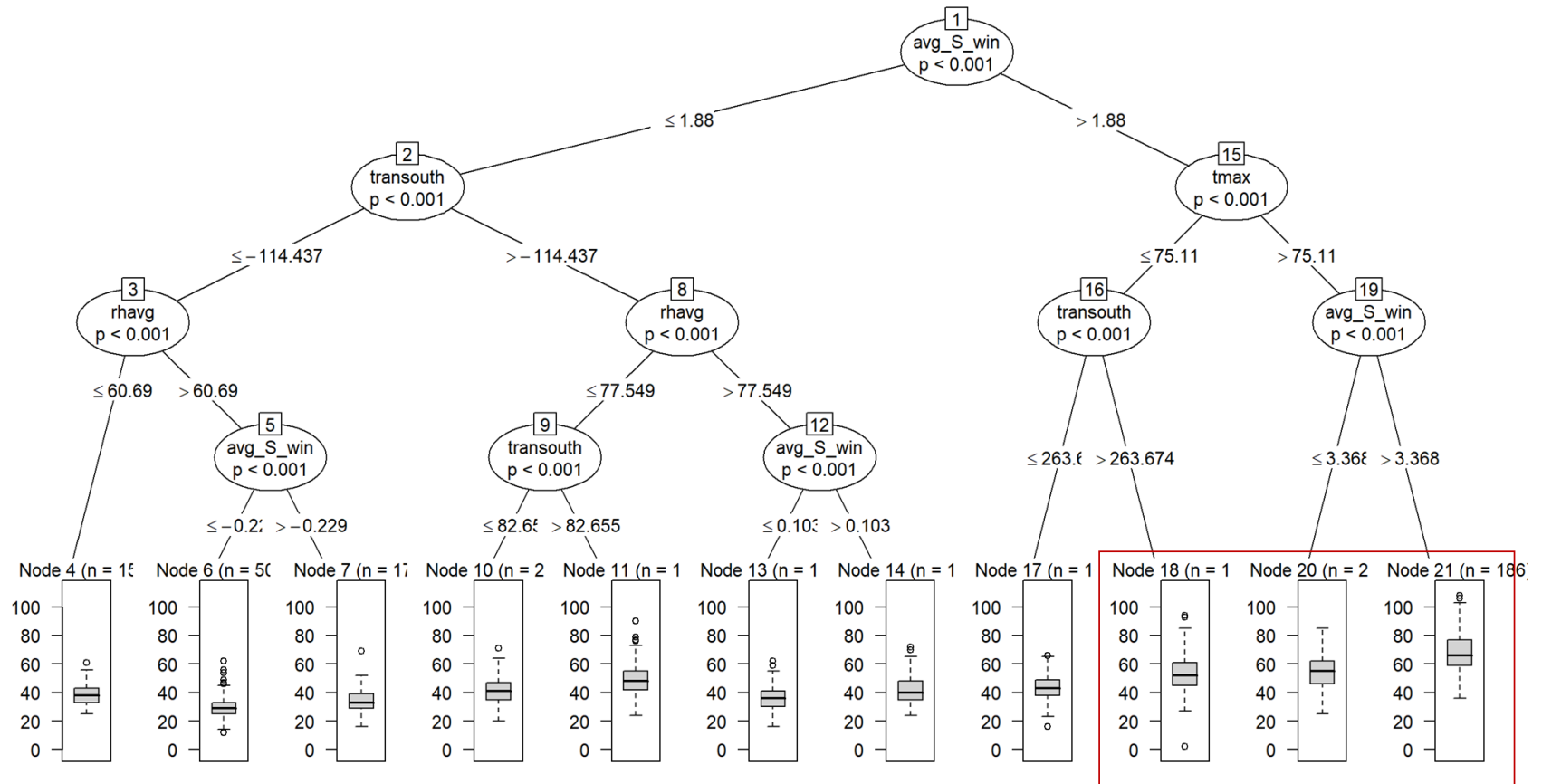
Figure A8.11. Classification and Regression Tree (CART) for the Door County monitor. The boxplots 17 at the bottom show the distribution of ozone concentrations on the different days in each node. The high-ozone nodes shown in the trends figure below (mean ozone >50 ppb) are outlined by the red boxes. See Table 1 in the main document for a description of the different variables.
