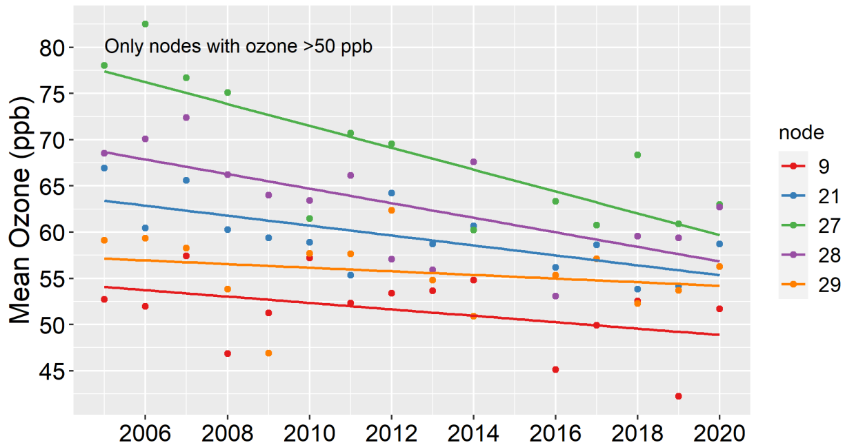
Figure A4.3. Trends in average (mean) ozone in high-ozone nodes for the Detroit monitors. High-ozone nodes are those with mean ozone concentrations over 50 ppb.
