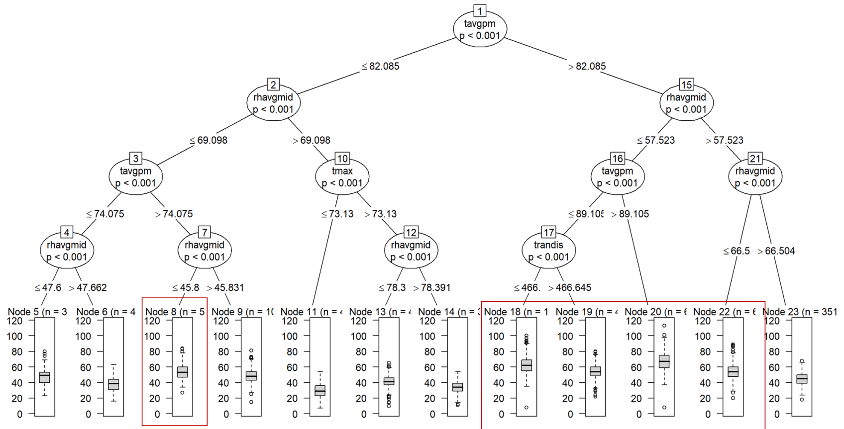
Figure A2.2. Classification and Regression Tree (CART) for the Cincinnati monitors. The boxplots 5 at the bottom show the distribution of ozone concentrations on the different days in each node. The high-ozone nodes shown in the trends figure below (mean ozone >50 ppb) are outlined by the red boxes. See Table 1 in the main document for a description of the different variables.
