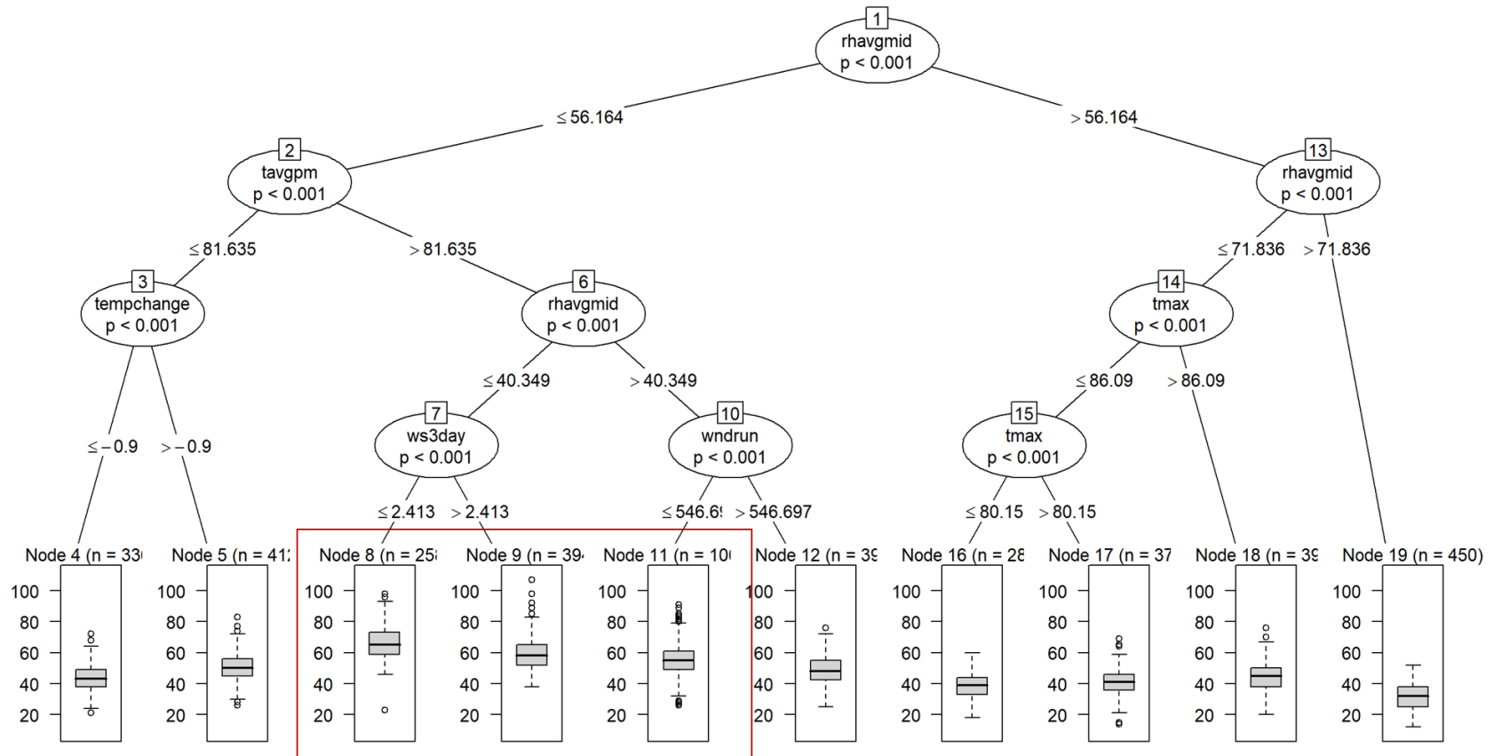
Figure A5.2. Classification and Regression Tree (CART) for the Louisville monitors. The boxplots 8 at the bottom show the distribution of ozone concentrations on the different days in each node. The high-ozone nodes shown in the trends figure below (mean ozone >50 ppb) are outlined by the red boxes. See Table 1 in the main document for a description of the different variables.
